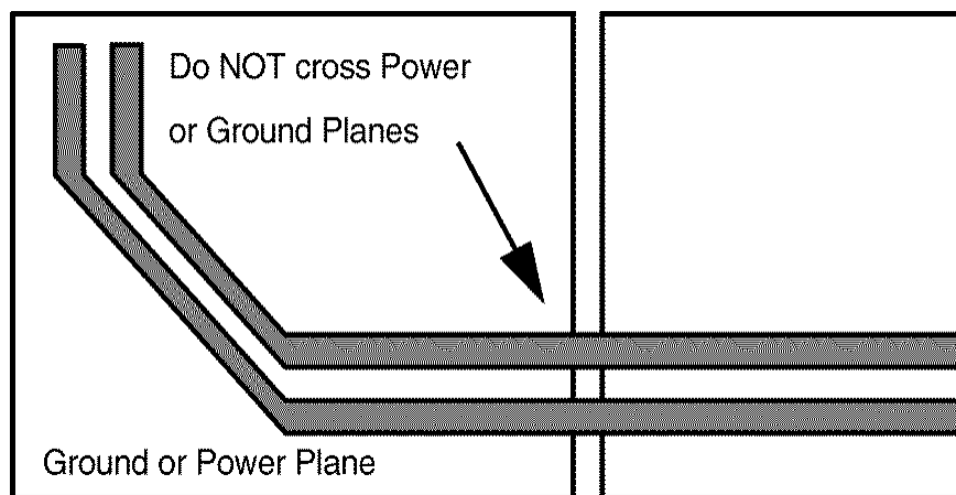
Figure 148. Power and Ground Plane Breaks
