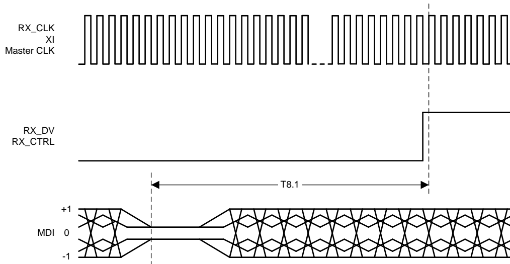
Figure 18. Receive Latency
